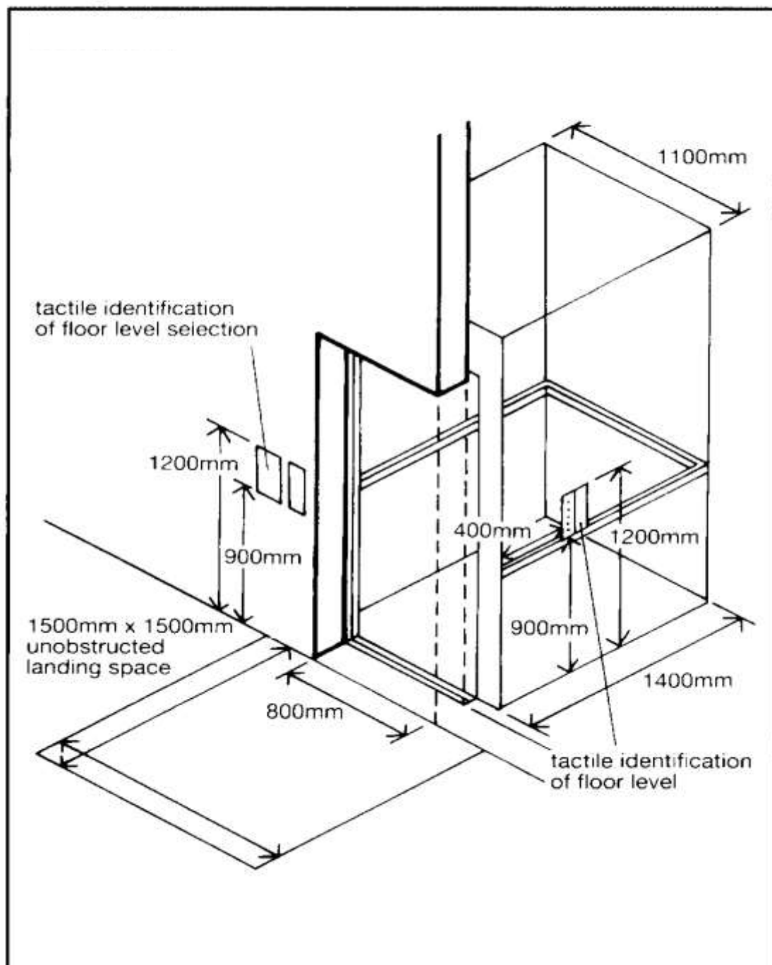
Diagram 11 Lift dimensions
